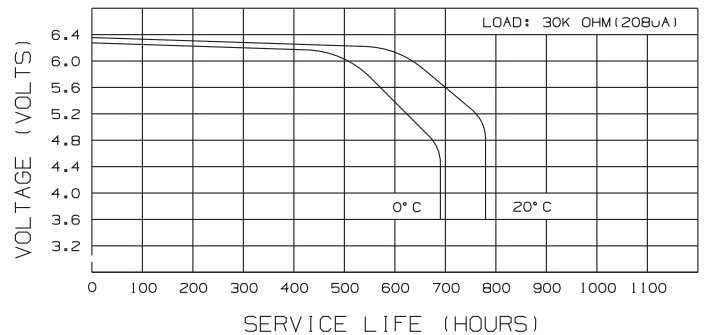
Typical Temperature Characteristics KS28
